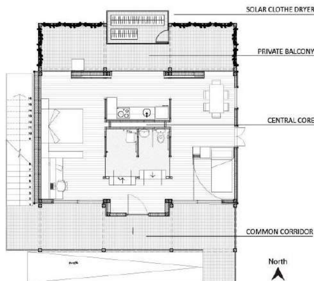
Figure 4. Floor plan "Tendal" housing prototype.
